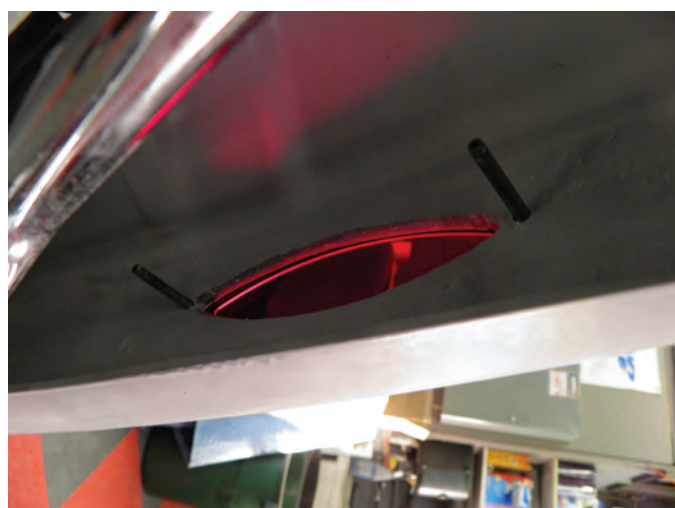
10. Slide the bezel with the set screws installed through the fender / bag and then slide the light box over the two studs and secure it with the two nuts provided.
