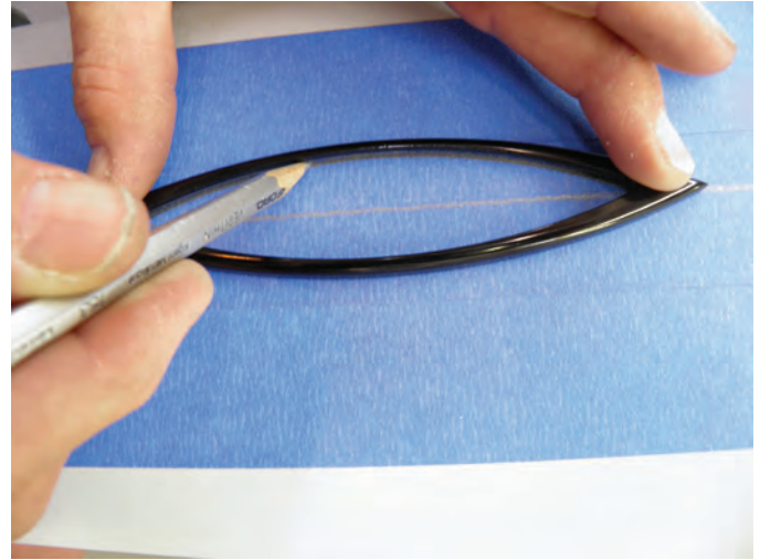
02. Trace the inside bezel and mark the two mounting hole locations. Drill the two mounting holes.
