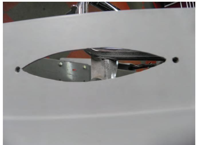
06. Our bezel is thin so make sure you cut to the inside of your line and then file the final shape.
